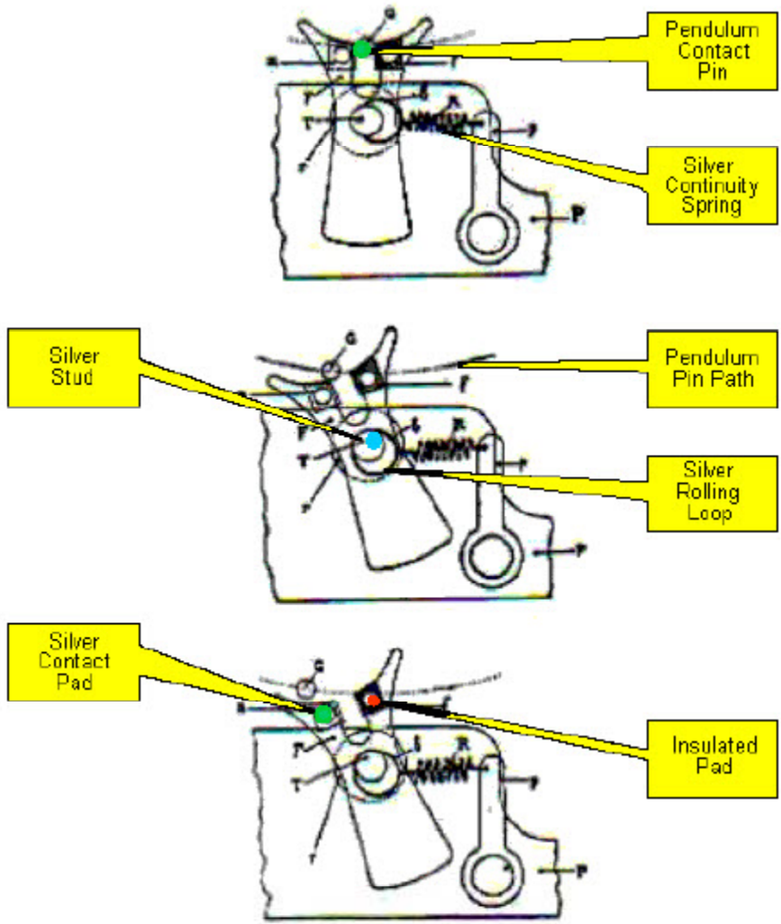
Fork and Pin Operation
