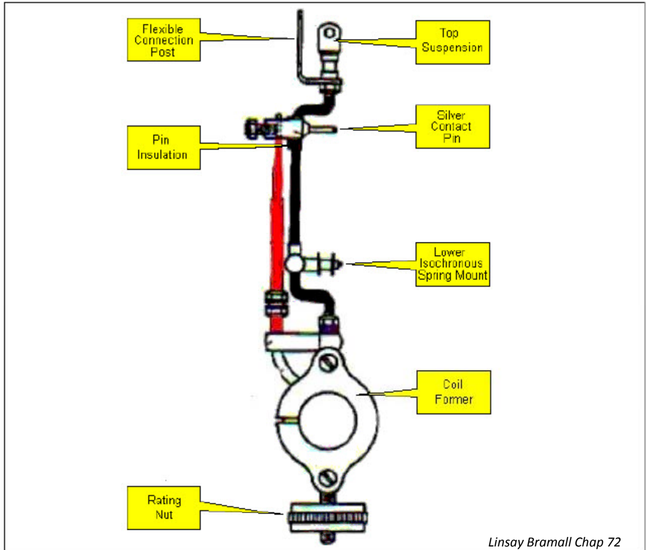
Pendulum Assembly
