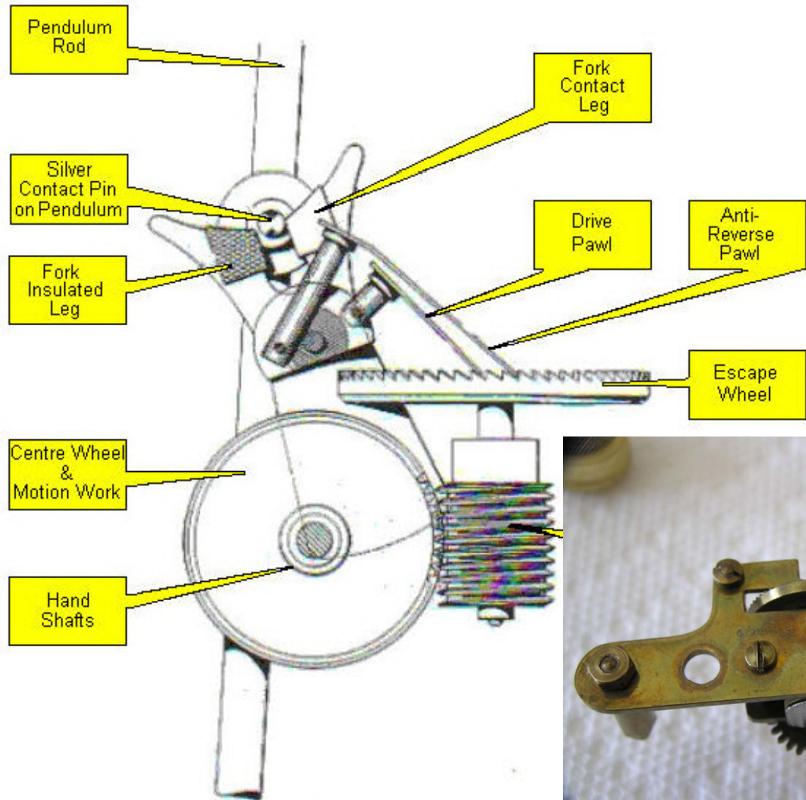
The Clock Movement
